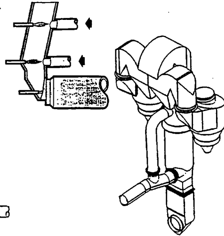
PREPOL®-MSC Multi-stage-combustion
